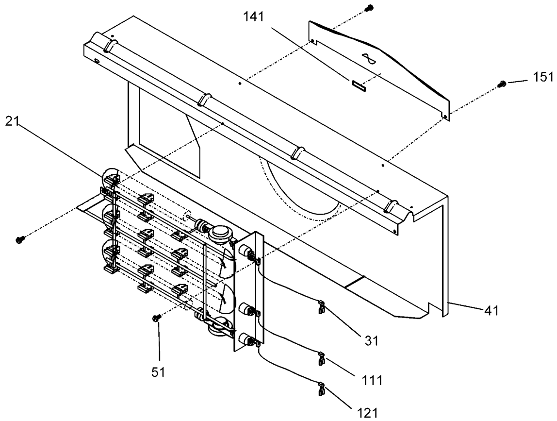
2 STAGE HEAT
